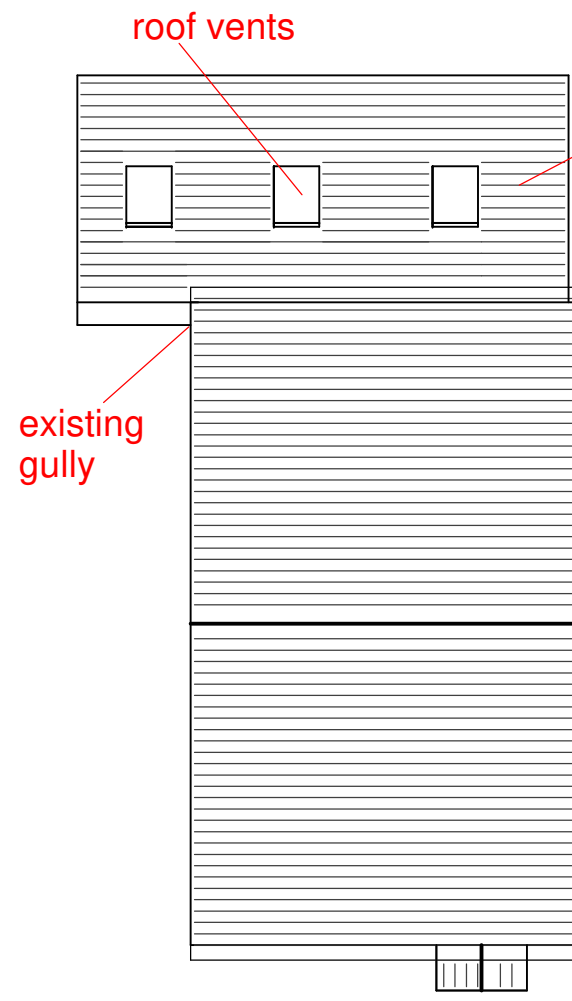
ROOF PLAN
