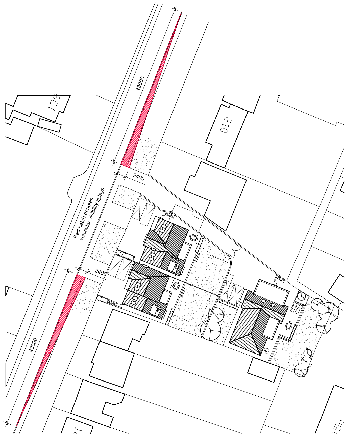
1. 43x2.4m Vehicular Visibility Splays
